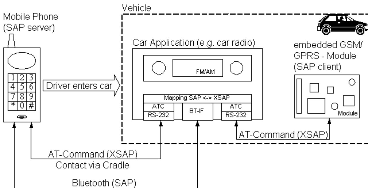
Figure 15.1: Basic Remote SIM Access Usage Scenario
