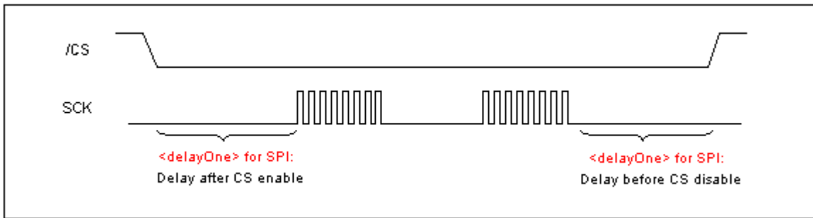
Figure 19.4: Delay time on SPI after/before CS enable/disable
