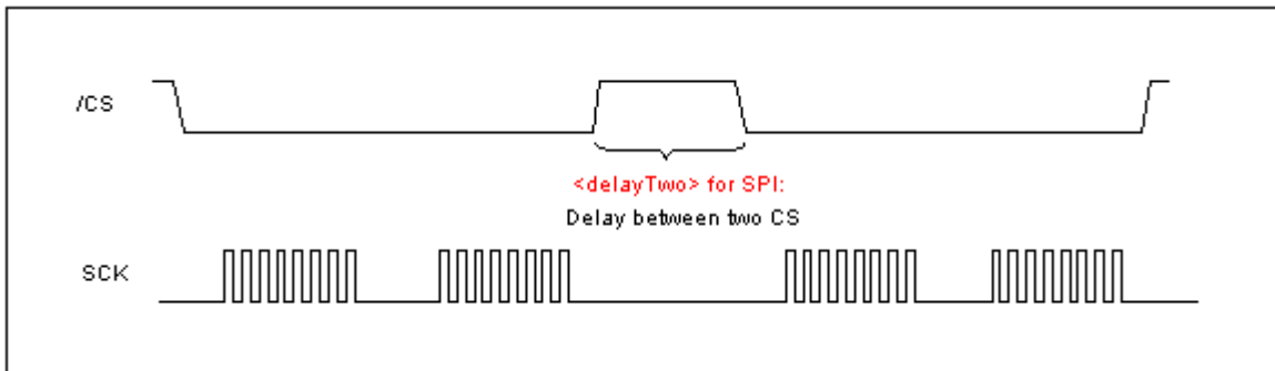
Figure 19.5: Delay time between two CS on SPI
