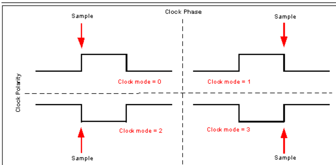
Figure 19.6: Clock modes selectable on SPI
