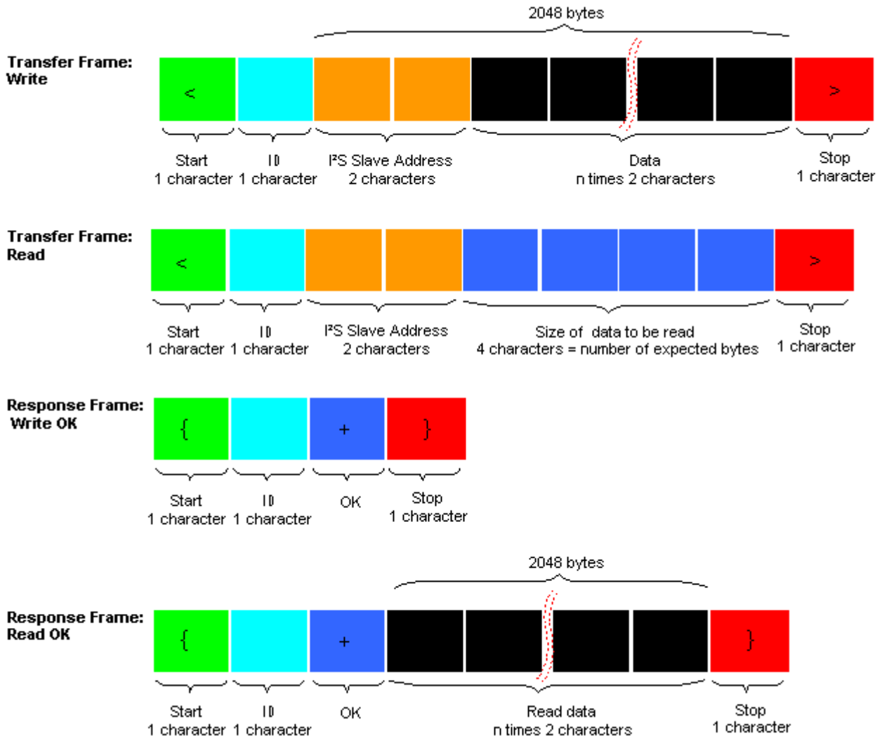
Figure 19.7: Number of characters in I 2 C Transfer and Response Frames
