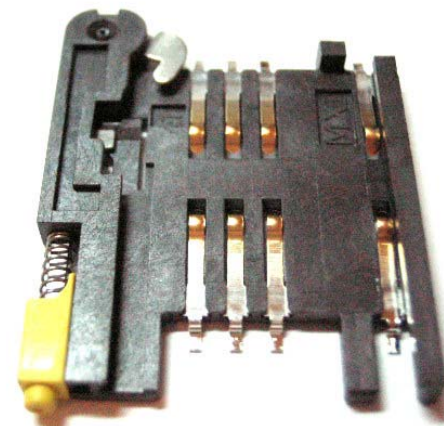
p/n : 91228-0001 SIM Card Holder ( Socket ) For All Modules
