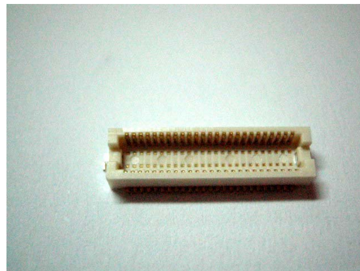
p/n : DF12(3.0)-50DP-0.5V(81) 50-pin board-board Connector Only for TC45/MC388/MC45
